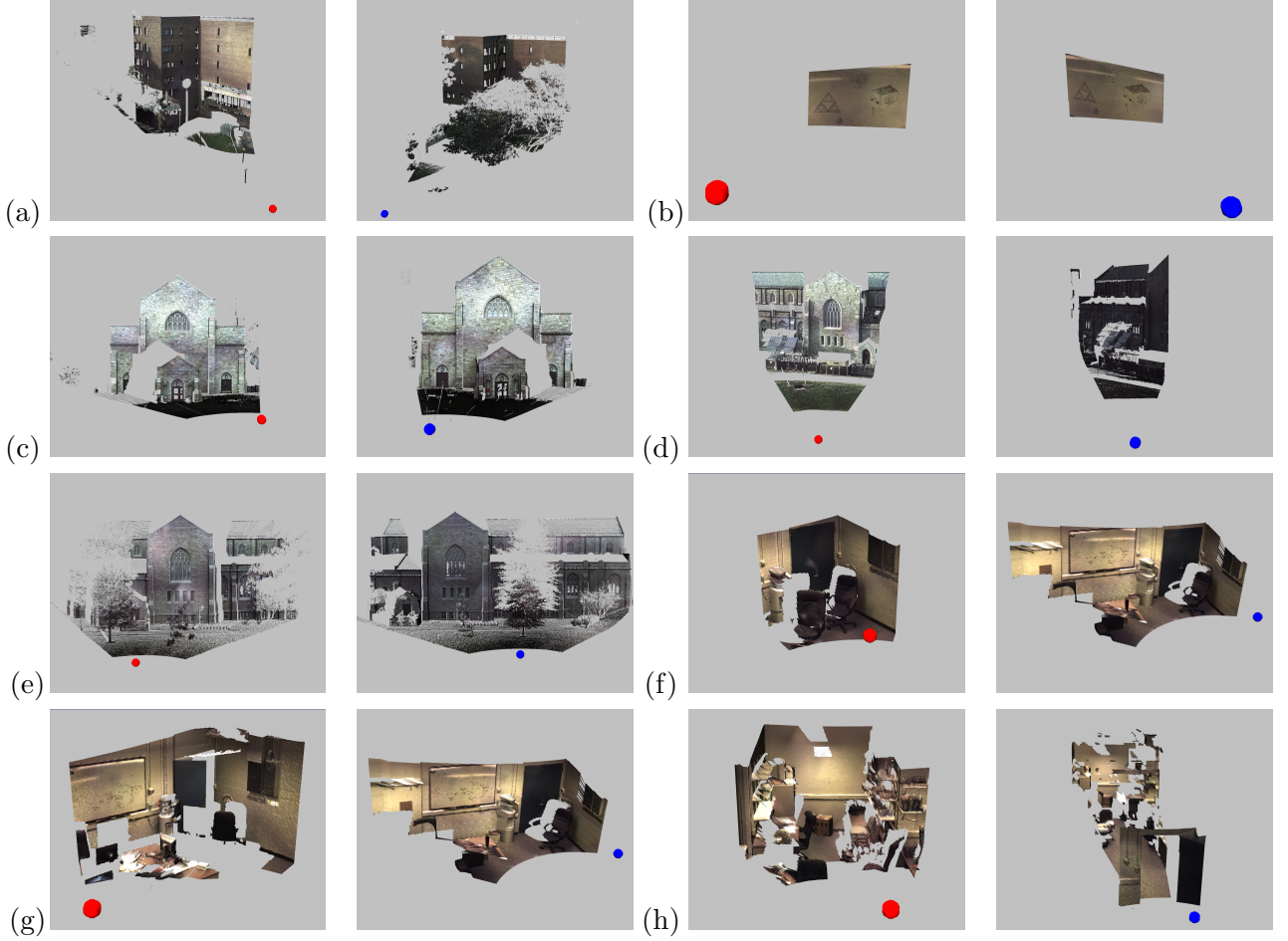
Fig. 10. (a) JEC – highly repetitive structure and large viewpoint difference. (b) Whiteboard – a flat scan that demonstrates the power of image-feature matching. (c) VCC West – easy pair, but has noisier images due to rain during the scanning. (d) VCC South – illumination differences and smaller overlap. (e) VCC North – easy pair, has one main overlapping face that provides many good initializations. (f) Lab Regular – indoor scan with varying viewpoints and smaller overlap. (g) Lab Large – indoor scan with varying viewpoints. (h) M336 into M301 – a difficult scan pair, it has a large sample spacing difference between scans, also a doorway blocks part of one scan’s view.
