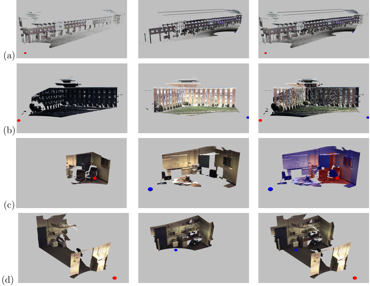
Fig. 9. These are the (a) BioTech, (b) Sci Center, (c) Lab Changes, and (d) M301 into M336 scan pairs. Scan pairs (a) and (b) have highly repetitive structure; the pair (b) is further complicated by illumination differences. Scan pair (c) demonstrates the algorithm’s ability to register scans with many changes; the right-hand picture is tinted to show the changes between the scans. The only overlapping parts between the two original scans are the walls and the water cooler. Scan pair (d) demonstrates the registration of the inside of a room and the same room seen through a doorway.
