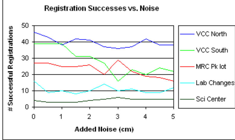
Fig. 11. Investigating the effect of additional noise on the performance of the algorithm. The number of registration successes in the top 50 initializations is plotted as a function of the standard deviation of the added noise variance for five representative scan pairs. The additional noise has little effect on the overall power of the algorithm because only a single success is needed per scan pair.
