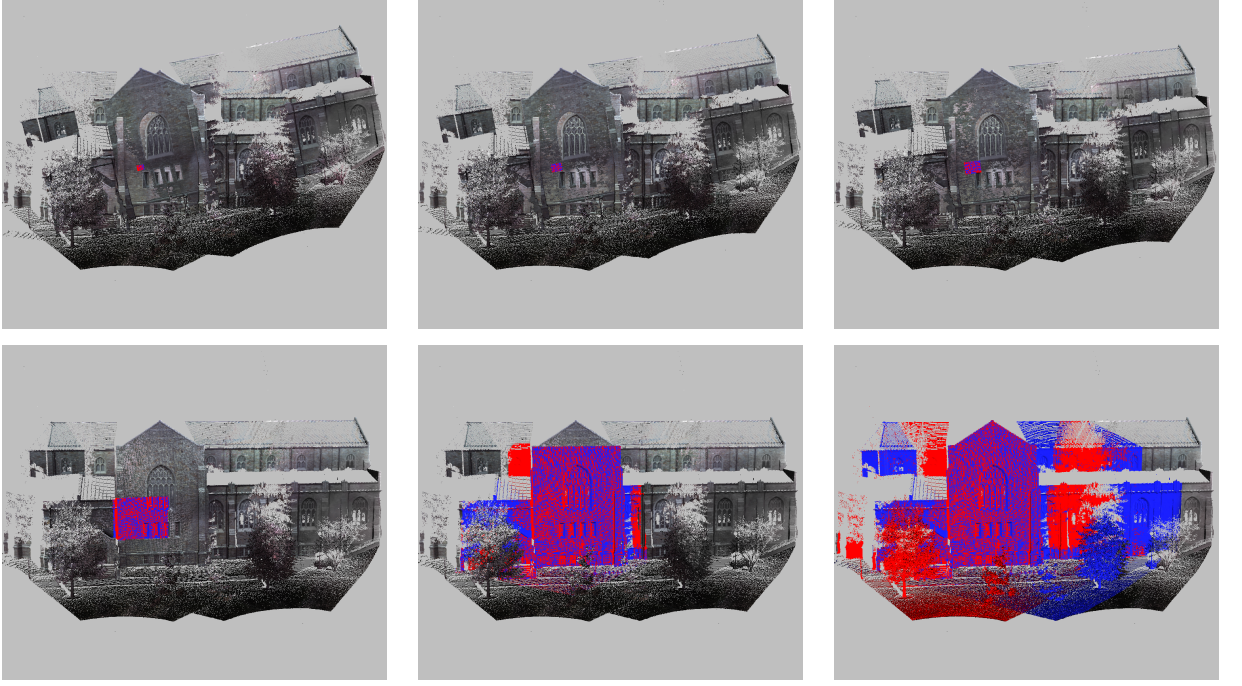
Fig. 6. Several iterations of ICP estimation and region growth of a relatively easy pair called “VCC North”. The colored regions represent the area inside the current bootstrap region, \Omega_t . The first frame shows the initial alignment of the scans and the initial region. Subsequent frames show the alignment and the region following iterations 1, 2, 5, 8, and 14 respectively. The correction of the strong initial misalignment can be clearly seen. Regions that are solidly one color or the other were only seen from the viewpoint of one scan.
