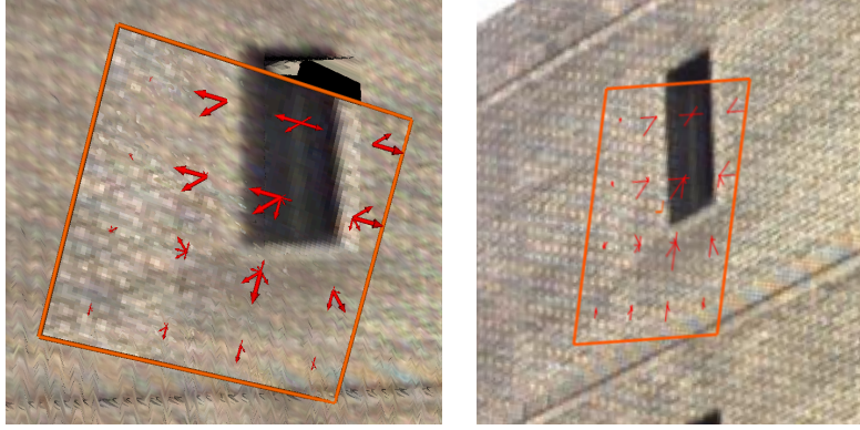
Fig. 5. Illustrating the computation of the augmented keypoint descriptor. The affine mapping from the surface tangent plane to the image plane determines a mapping between a square grid on the surface and an affine grid in the image. On the left the augmented keypoint descriptor is shown on the range plane it is computed on – the affine approximation is visible here since the descriptor region is not a perfect square. The right image shows the descriptor region projected into the image plane.
