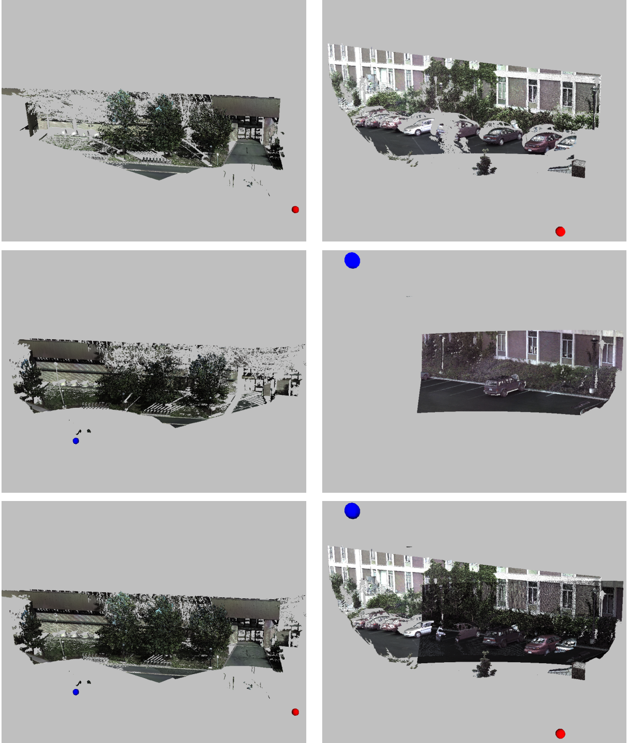
Fig. 1. Two example challenging pairs that our algorithm registers (DCC and MRC Parking lot). The top and center of the left column show a pair of scans taken from vastly different viewpoints, in which trees occlude much of the common structure. The top and center of the right column show two scans of a parking lot and building where all of the vehicles are different between the two scans. In both cases, as shown on the bottom, the algorithm automatically and accurately aligned the scans. The spheres in the figures indicate the scanner's location.
